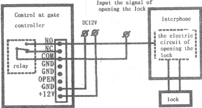
The map of circuit
