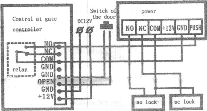
The map of circuit (use alone )
